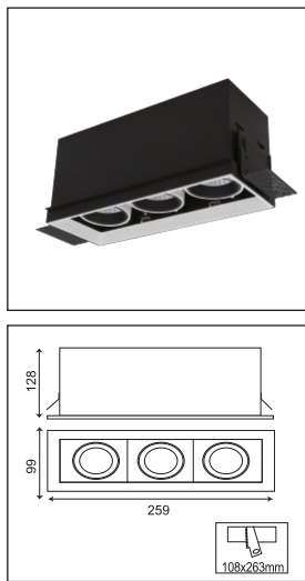
A - Ø 259X99*128mm
